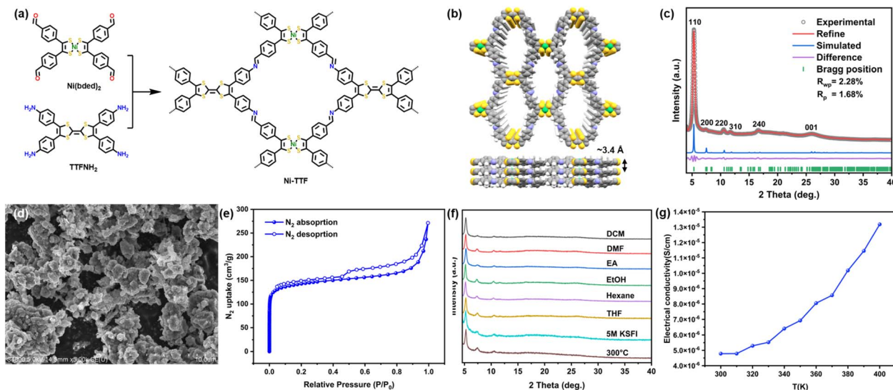
Fig. 1 (a) Synthesis of Ni-TTF. (b) Top and side views of the simulated structure of Ni-TTF. (c) Pawley refinement and the PXR D pattern of Ni-TTF. (d) HRTEM image of Ni-TTF. (e) N_2 adsorption/desorption isotherm of Ni-TTF. (f) PXR D patterns showing stability of Ni-TTF. (g) Temperature dependent conductivity of Ni-TTF from 300 K to 400 K.
