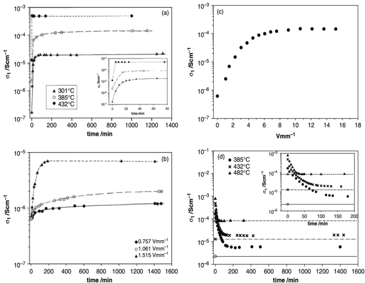
Fig. 2 Bulk conductivity of \text{BaTi}_{0.99}\text{O}_{2.98} (a) at different temperatures and times with a voltage of 10 V and field 15.1 \text{Vmm}^{-1} , (b) at different voltages and times at 335 °C, (c) limiting conductivity for different voltages at 335 °C and (d) recovery at different temperatures on removal of the bias voltage (horizontal lines indicate the initial conductivity before voltage application); reproduced from H. Beltran et al. , J. Am. Ceram. Soc. , 2011, 94, 2951 with permission from Wiley publishing.
