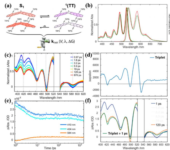
Fig. 11 (a) Illustration of electronic coupling strength in the S_1 and ^1(\text{TT}) states for dimers 37 and 38 . (b) Normalized steady-state electronic absorption (solid) and emission (dashed) spectra for dimers 37 (red) and 38 (green) in toluene. (c) TA spectra of dimer 38 in toluene following ultrafast excitation at 530 nm. The spectral region around the excitation wavelength is removed due to pump scatter. (d) Triplet \Delta\epsilon spectrum for dimer 38 from sensitization experiment in toluene. (e) Selected single wavelength kinetic traces (data points) taken from the full-spectrum data with applied model fits (lines) retrieved from global analysis. (f) Selected spectral slices for dimer 38 at 1 ps (blue) and 120 ps (red) along with a reconstructed TA spectrum (green), which is comprised of a superposition between the 1 ps TA spectrum and the sensitized triplet \Delta\epsilon spectrum from (d). Reproduced with permission. 123 Copyright 2019, the American Chemical Society.
