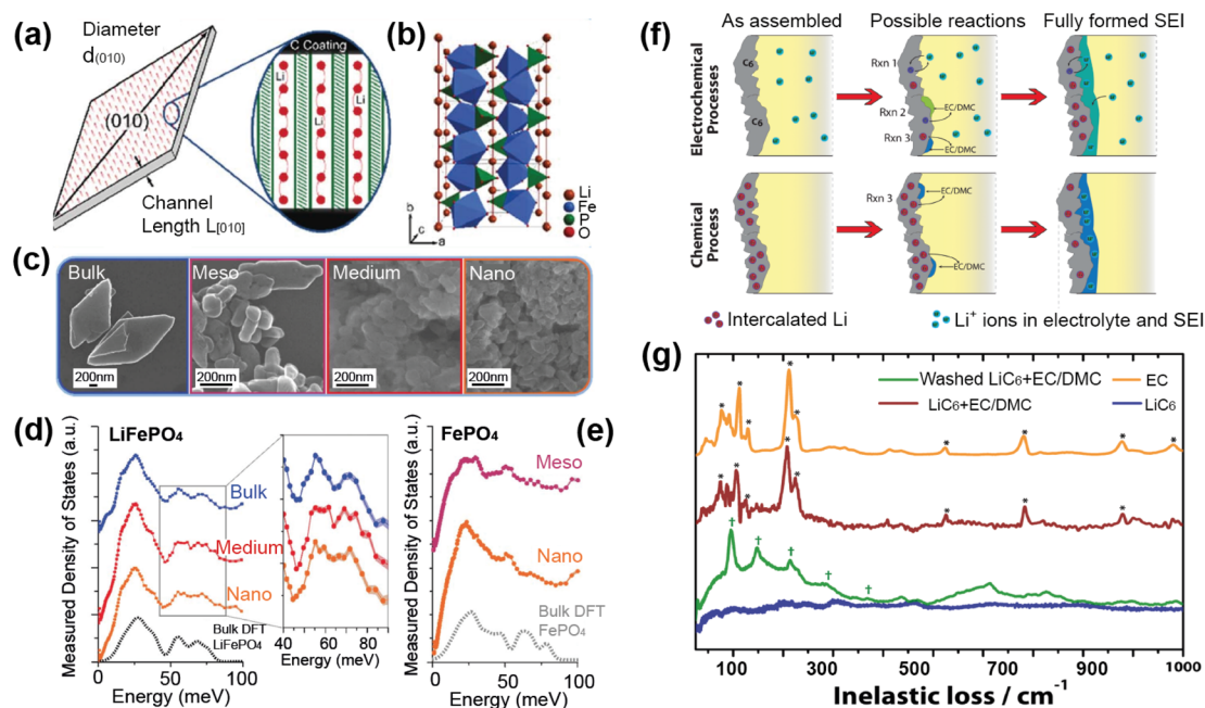
Fig. 22 Platelet shape (a), structure (b), and SEM images (c) of LiFePO 4 (LFP) particles with the INS spectra of the lithiated and delithiated samples shown in (d) and (e), respectively. Reproduced from ref. 104 with permission from the Royal Society of Chemistry. (f) Schematic of the different strategies for forming an SEI along with the types of reactions involved. (g) Inelastic neutron scattering of EC, LiC 6 + EC/DMC, and washed LiC 6 + EC/DMC. Asterisks indicate major peaks ascribed to EC and daggers correspond to peak locations of poly(ethylene oxide)-type vibrations. Reprinted with permission from ref. 105 Copyright (2015) American Chemical Society.
