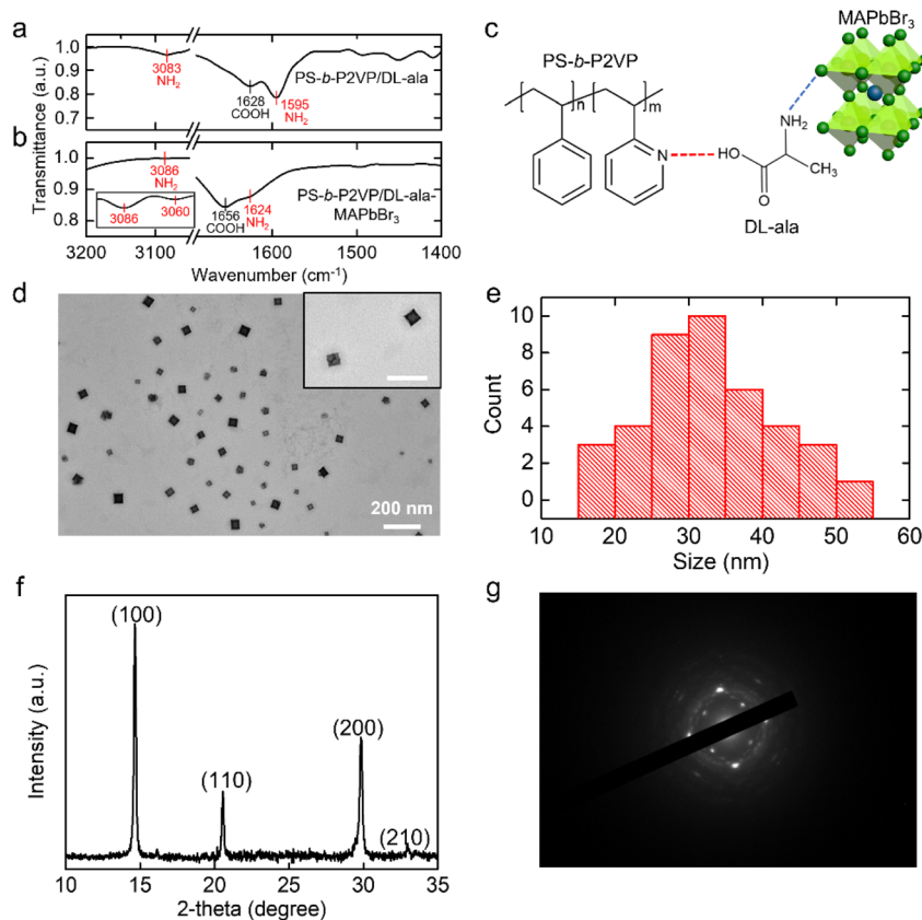
Fig. 2 FTIR spectra of (a) PS-b-P2VP/DL-ala and (b) PS-b-P2VP/DL-ala inverse micelle-encapsulated \text{MAPbBr}_3 NCs. (c) Molecular structures showing the chemical interactions among PS-b-P2VP , DL-ala , and \text{MAPbBr}_3 NCs. (d) TEM image (inset: high-magnification TEM image, scale bar: 100 nm), (e) size distribution histogram (average size: 32.7 nm), (f) XRD pattern, and (g) the SAED pattern of the PS-b-P2VP/DL-ala inverse micelle-encapsulated \text{MAPbBr}_3 NCs.
