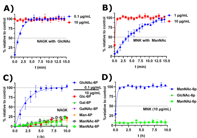
Fig. 6 (A and B) Real-time ^{31}\text{P} -HMBC-NMR of the phosphorylation (ATP 5 mM) of GlcNAc and ManNAc ( 400 \mu\text{M} ) by NAGK and MNK at different concentrations - nonlinear fit data in ESI† Table 13 and 14. (C and D) Real-time ^{31}\text{P} -HMBC-NMR of the phosphorylation of different carbohydrates ( 400 \mu\text{M} ) by NAGK and MNK with ATP (5 mM) - nonlinear fit data in ESI† Tables 15 and 16.
