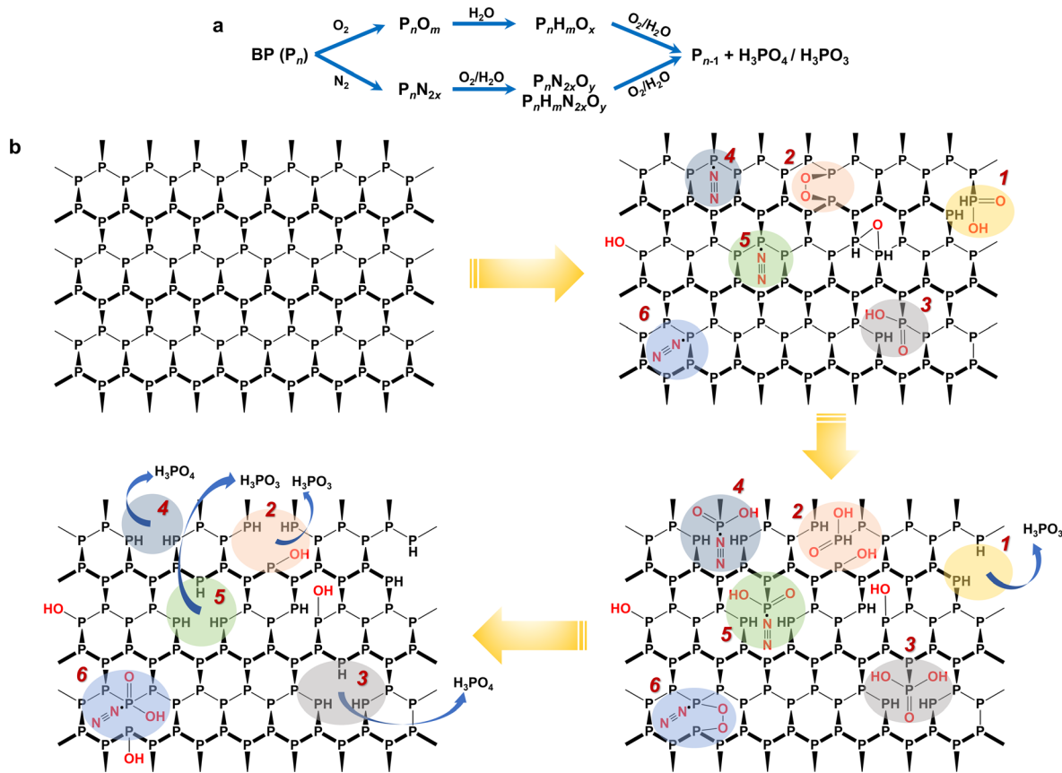
Fig. 3 Proposed degradation pathways of BP in the ambient environment based on LDI-MS fingerprinting results. (a) Two general pathways for BP degradation, direct oxidation and \text{N}_2 -addition oxidation. (b) Molecular structural description of degradation of BP in the ambient environment. The colored shadows indicate different degradation routes. 1, 2, 3: direct oxidation, and 4, 5 and 6: \text{N}_2 -addition oxidation. All degradation routes were deduced from the MS fingerprinting in Fig. 2, and the corresponding feature peaks are given in Table S6.† Note: this figure only shows the pathways and intermediates derived from the MS fingerprints and may not include all possible degradation pathways.
