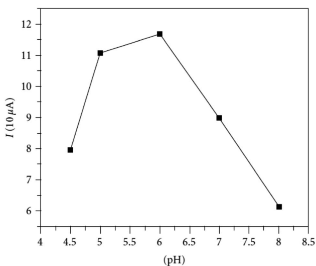
Fig. 11 pH effect of parathion ( 3.43 \times 10^{-5} M) on peak current at fabricated poly(safranine) film under scan rate: 100 \text{ mV s}^{-1} . This figure has been adapted/reproduced from ref. 35 with permission from Hindawi, copyright (2023).
