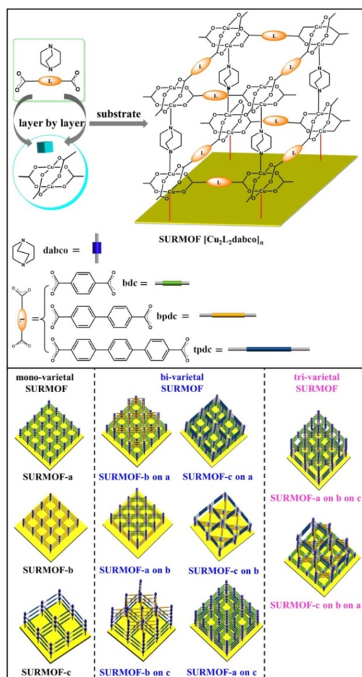
Scheme 1 Schematic illustration for the preparation of mono-varietal SURMOFs [\text{Cu}_2\text{L}_2\text{dabco}]_n ( \text{L} = \text{bdc} , \text{bpdc} , and \text{tpdc} ) and their multiple (bi-varietal and tri-varietal) SURMOFs on substrate surfaces by using a LPE layer by layer method.
