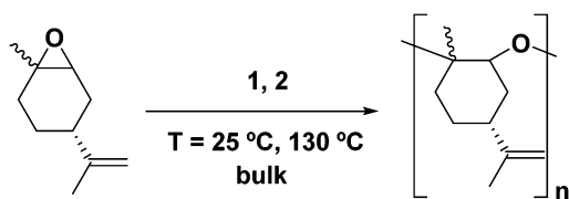
Scheme 1 Catalytic polymerization of (+)-limonene oxide.
