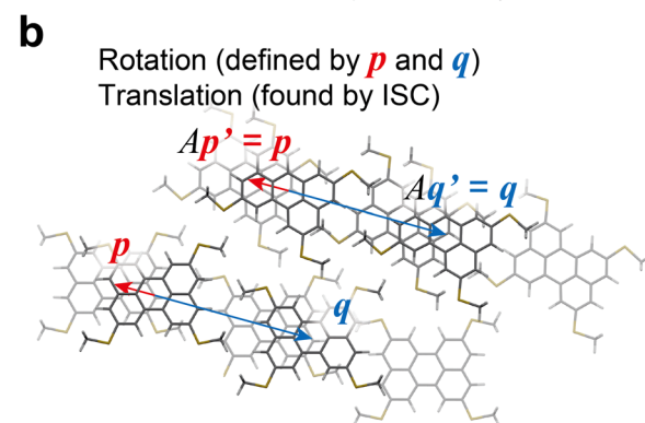
Fig. 4 Construction of the neighboring layer in the iBW structure of MT-perylene from the BW structure. The mirror plane can be chosen arbitrarily and is y = 8.5 Å in the present case (a). Rotation matrix A in (b) is defined in eqn (1) to ensure A\mathbf{q}' = \mathbf{q} (and A\mathbf{p}' = \mathbf{p} ).
