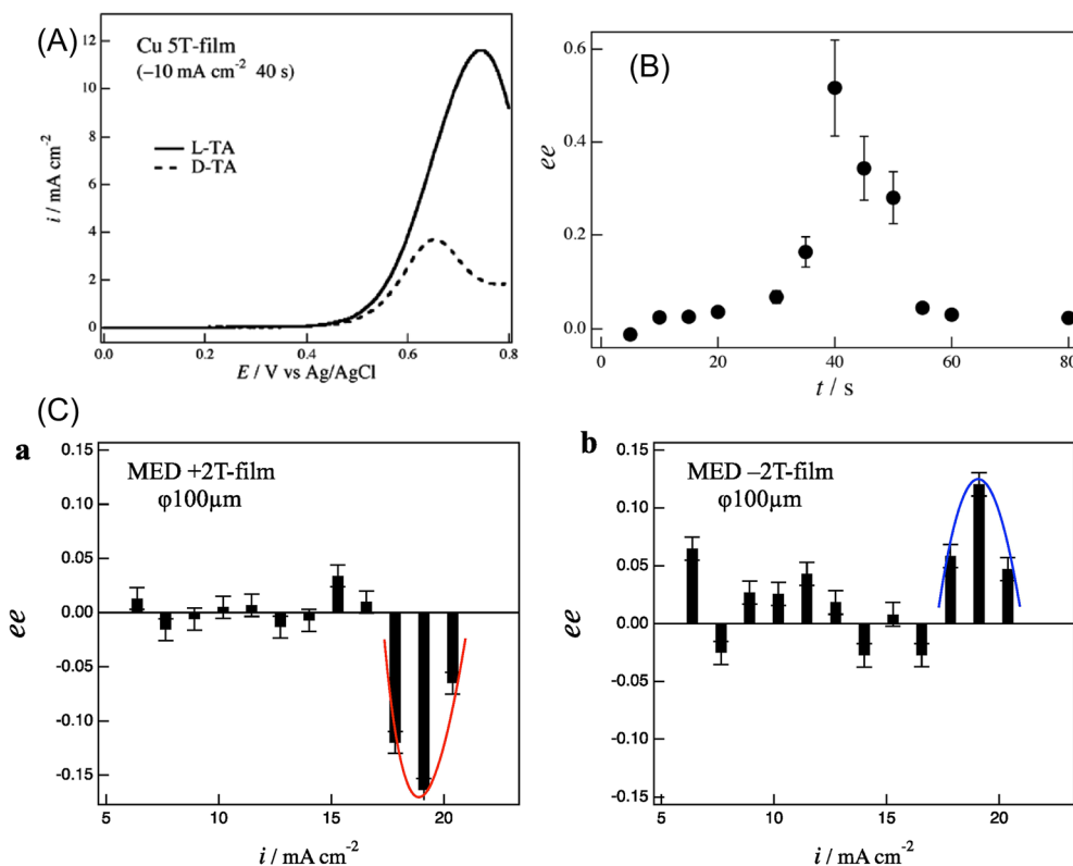
Fig. 21 (A) Voltammograms of 20 mM L- and D-tartaric acid (TA) under 50 mV s^{-1} in Cu 5 T-film electrode in 0.1 M NaOH with 40 s deposition time. 259 (B) Enantioexcess ( ee ) vs. magneto-electrodeposition time. Reprinted with permission from ref. 259. Copyright © 2014, The Polish Physical Society. (C) ee ratio vs. deposition current on a 100 \mu m electrode: (a) +2 T film and (b) -2 T film. Reprinted from ref. 277.
