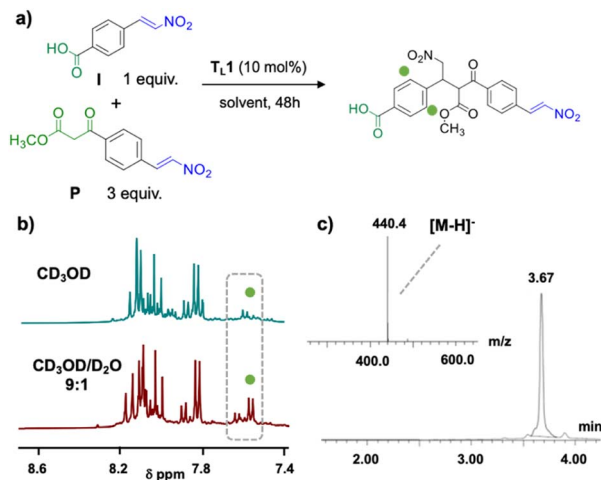
Fig. 5 (a) Catalytic templated oligomerization with T_L1 ; (b) ^1\text{H} NMR spectra (selected region) of the reaction in \text{CD}_3\text{OD} (top) and \text{CD}_3\text{OD}/\text{D}_2\text{O} 9 : 1 (bottom) recorded after 24 h – signals corresponding to the product are labelled with a green dot; and (c) LC-MS analysis of the precipitate formed in the reaction in \text{CD}_3\text{OD}/\text{D}_2\text{O} 9 : 1 (inset: ESI ^- spectrum of the peak at 3.67 min).
