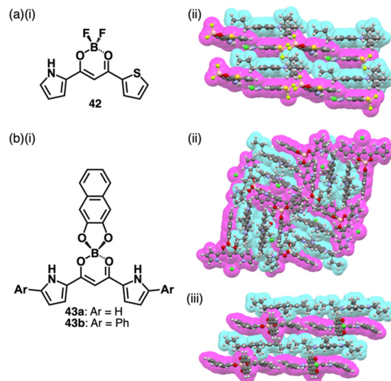
Fig. 29 (a) (i) Pyrrolylthienyldiketone BF_2 complex 42 and (ii) single-crystal X-ray structure of {}^3TATA^+-42_2\cdot Cl^- and (b) (i) naphthalenediolate boron complexes 43a,b and (ii) single-crystal X-ray structures of {}^3TATA^+-43a\cdot Cl^- and (iii) {}^3TATA^+-43b\cdot Cl^- . The crystal structures are redrawn from cif files: 1840326, 2227398 and 2227399.
