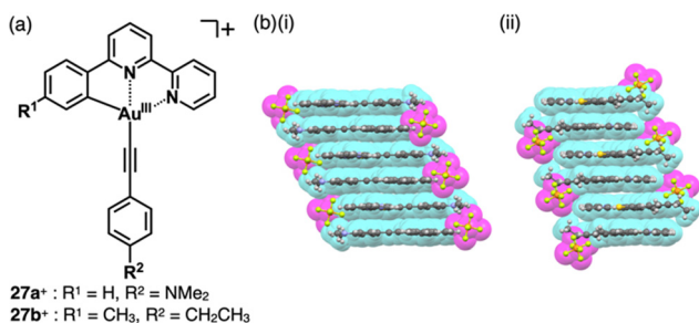
Fig. 17 (a) Positively charged phenylbipyridine \text{Au}^{\text{III}} complexes 27\text{a},\text{b}^+ and (b) single-crystal X-ray structures of (i) 27\text{a}^+-\text{PF}_6^- and (ii) 27\text{b}^+-\text{PF}_6^- (redrawn from cif files: 841764 and 897336).
