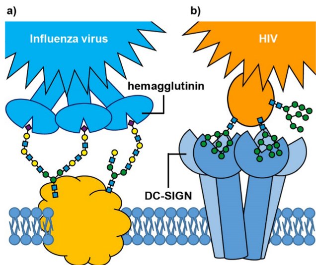
Fig. 1 Glycan-mediated cell targeting: (a) influenza virus hemagglutinin binds to multiple sialic acids on cell surface glycoproteins; (b) cell surface DC-SIGN receptor binds to mannose on the surface of HIV.
