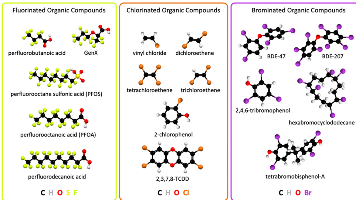
Fig. 1 Chemical structures of widespread halogenated organic water pollutants; 2,3,7,8-TCDD, 2,3,7,8-tetrachlorodibenzodioxin; BDE, bromodiphenyl ether.
