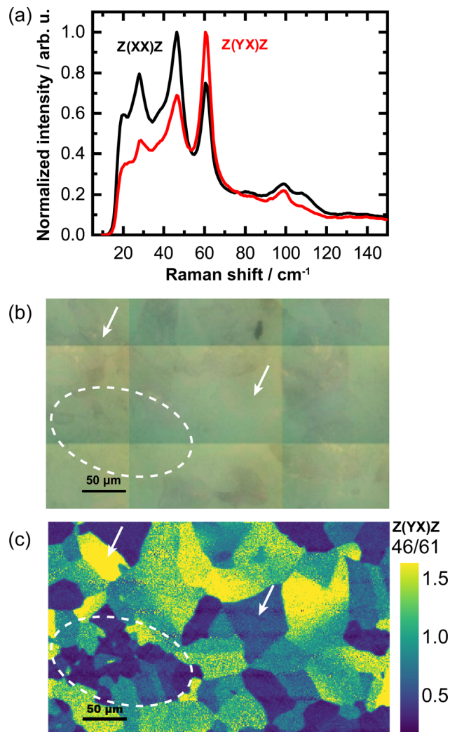
Fig. 4 (a) Average polarised Raman spectra of \text{PDMAPbI}_4 measured in the Z(\text{XX})Z and Z(\text{YX})Z configuration, where the terms inside the brackets indicate the polarisation direction of the incident and detected light, respectively. (b) White light micrograph of the area on which Raman maps were acquired. (c) False colour map showing the ratio of the intensity of the 46\text{ cm}^{-1} peak over the 61\text{ cm}^{-1} peak for the Z(\text{YX})Z polarisation.
