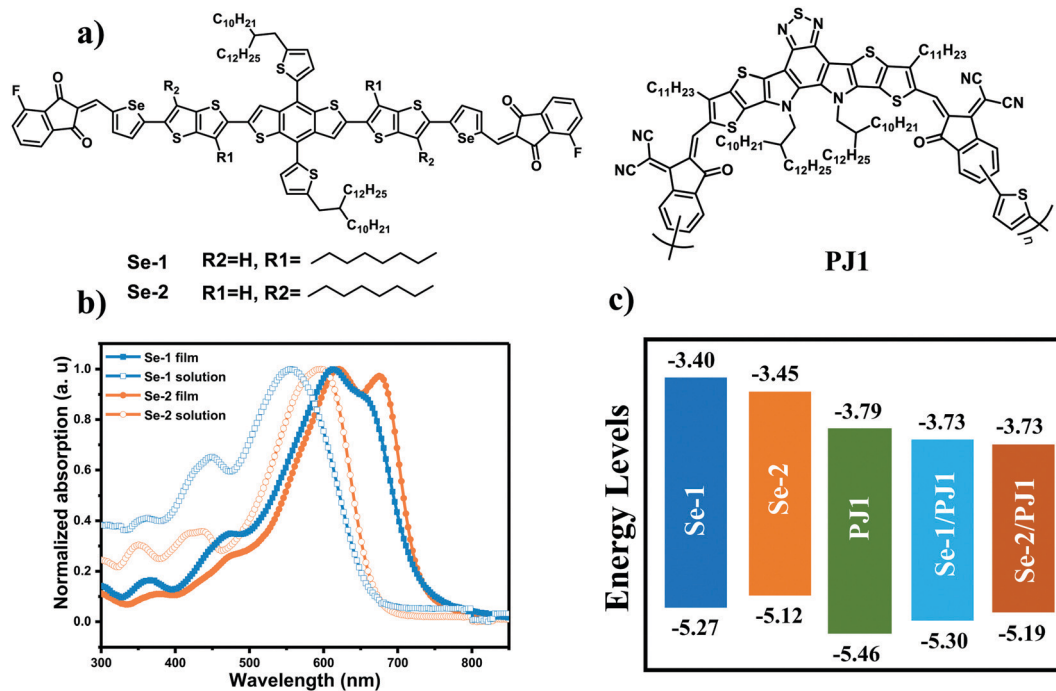
Fig. 1 Molecule properties: (a) molecule structures of donors and polymer acceptors; (b) absorption spectrum of small molecules; (c) energy level alignment of small molecules and polymer acceptor in pristine and blend film.
