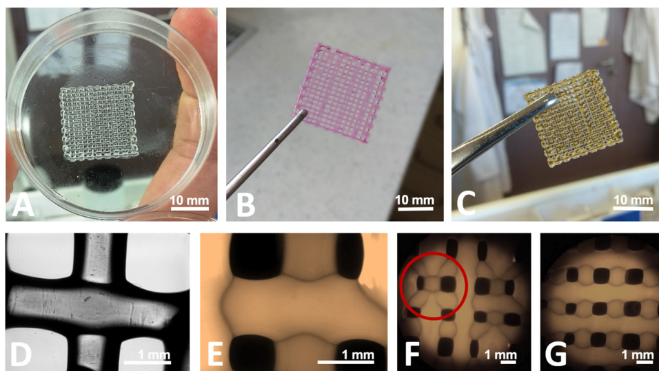
Fig. 2 3D bioprinted gelatin–alginate hydrogel (gelatin 0.2 \text{ g mL}^{-1} , sodium alginate 0.04 \text{ g mL}^{-1} ) matrices before lyophilization – (A)–(C) phone camera pictures: (A) immediately after printing, bioink without additives, no cross-linking, (B) bioink with rhodamine, no cross-linking, (C) bioink without additives, after cross-linking with 2% \text{Ca}^{2+} and 25% GTA solutions; (D) optical microscopy picture, magnification 200\times , bioink without additives, after cross-linking with 2% \text{Ca}^{2+} and 25% GTA solutions; (E) and (F) fluorescent microscopy pictures, bioink without additives, after cross-linking with 2% \text{Ca}^{2+} and 25% GTA solutions: (E) magnification 200\times , (F) magnification 20\times , (G) fluorescent microscopy picture, magnification 20\times , bioink without additives, after cross-linking with 25% GTA solution.
