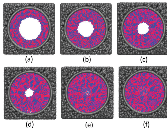
Fig. 3 The trajectory snapshots of conformation changes for the system of length 40 and grafting density 0.212 under highly acidic conditions, (a)step 0; (b) step 50 000; (c) step 100 000 (d) step 150 000; (e) step 200 000; and (f) step 250 000.
