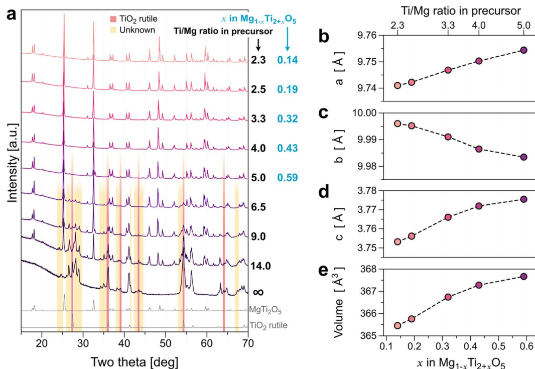
Fig. 3 (a) Series of XRD results of MTO synthesized from precursor with a \text{TiO}_2 content greater than \text{Ti/Mg} = 2.3 . Note that the remaining \text{TiO}_2 rutile phase (indicated by the red box) appears in MTOs ( \text{Ti/Mg} > 4.0 ) from the excessive Ti in the precursor. (b–e) Relations between the unit-cell parameters and volume as a function of x in \text{Mg}_{1-x}\text{Ti}_{2+x}\text{O}_5 .
