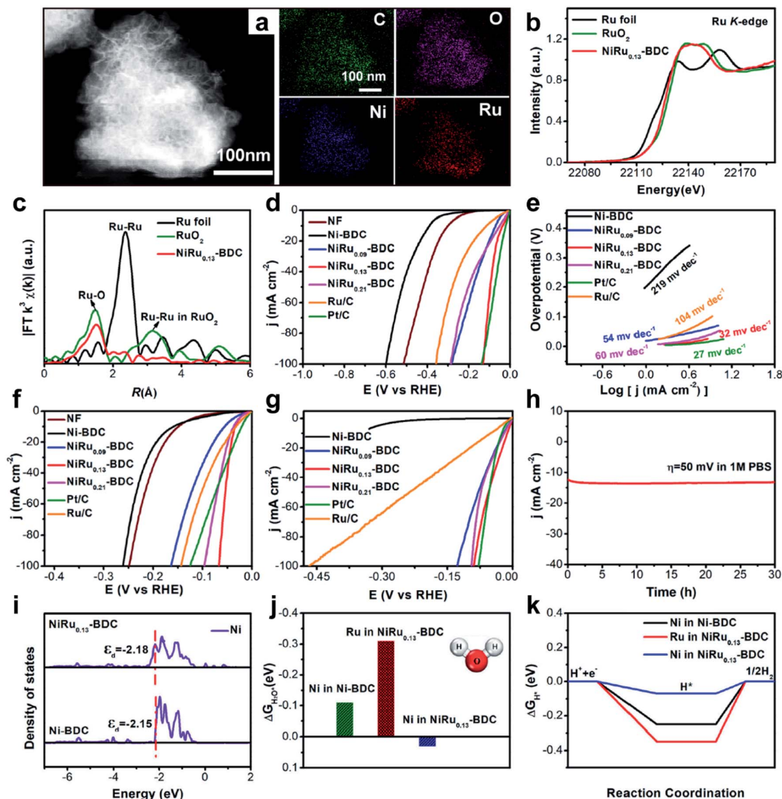
Fig. 12 (a) HAADF-STEM image and the corresponding STEM-EDXS elemental maps of \text{NiRu}_{0.13}\text{-BDC} . (b) Ru K-edge XANES spectra and (c) FT-EXAFS spectra of \text{NiRu}_{0.13}\text{-BDC} , Ru foil and \text{RuO}_2 . (d) LSV curves toward HER and (e) Tafel plots of Ni-BDC, \text{NiRu}_{0.09}\text{-BDC} , \text{NiRu}_{0.13}\text{-BDC} , \text{NiRu}_{0.21}\text{-BDC} in 1 M PBS; LSV curves of Ni-BDC, \text{NiRu}_{0.09}\text{-BDC} , \text{NiRu}_{0.13}\text{-BDC} , \text{NiRu}_{0.21}\text{-BDC} toward HER in (f) 1 M KOH and (g) 1 M HCl. (h) Chronoamperometric curves of \text{NiRu}_{0.13}\text{-BDC} in 1 M PBS. (i) Calculated DOS of Ni in Ni-BDC and \text{NiRu}_{0.13}\text{-BDC} ; (j) the calculated adsorption free energy of water and (k) \Delta G_{\text{H}^+} diagram of Ru in \text{NiRu}_{0.13}\text{-BDC} compared with Ni in Ni-BDC and \text{NiRu}_{0.13}\text{-BDC} . Reprinted with permission from ref. 33. Copyright 2021 Nature Publishing Group.
