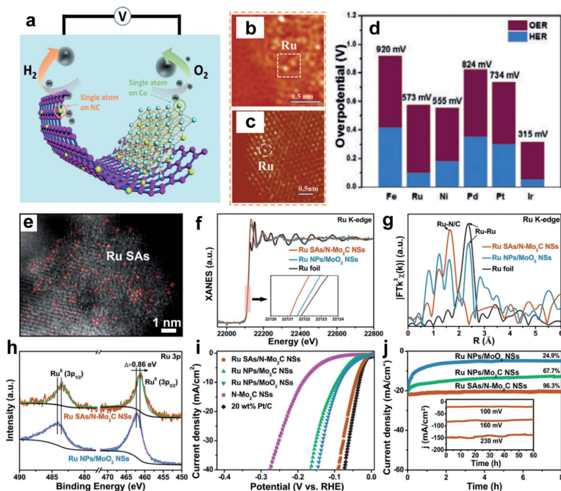
Fig. 13 (a) Illustration of the working mechanism of the prepared electrodes. FFT-1D HAADF images of Ru SA (b) on NC and (c) on Co particles. (d) The overall \eta_{10} of Fe SA @Co/NC, Ru SA @Co/NC, Ni SA @Co/NC, Pd SA @Co/NC, Pt SA @Co/NC and Ir SA @Co/NC in N 2 -saturated 1.0 M KOH. Reprinted with permission from ref. 30. Copyright 2019 John Wiley and Sons. (e) AC HAADF-STEM image of Ru SAs/N-Mo 3 C NSs. (f) XANES spectra and (g) k 3 -weighted FT-EXAFS spectra for Ru K-edge of Ru NPs/MoO 3 NSs, Ru SAs/N-Mo 3 C NSs and Ru foil. (h) High-resolution XPS spectra of Ru 3d for Ru NPs/MoO 3 NSs and Ru SAs/N-Mo 3 C NSs. (i) HER polarization curves and (j) time-dependent current density curves in 1.0 M KOH. Reprinted with permission from ref. 27. Copyright 2020 Elsevier.
