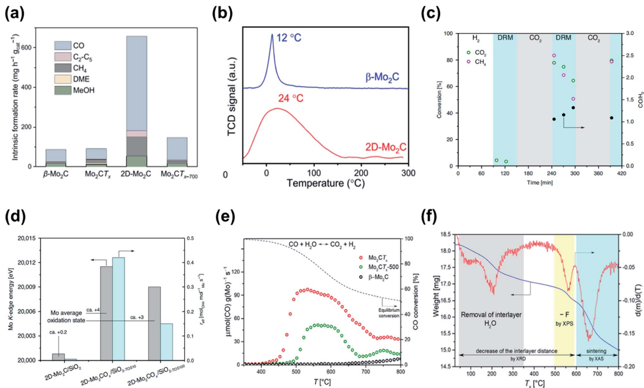
Fig. 8 The thermal catalysis with Mo 2 CT x . (a) Intrinsic formation rates of β-Mo 2 C, Mo 2 CT x , 2D-Mo 2 C, and Mo 2 CT x-700 . (b) CO temperature-programmed desorption (TPD) of 2D-Mo 2 C and β-Mo 2 C. Reproduced with permission. 51 Copyright 2021, Springer Nature. (c) Catalytic performance of 2D-Mo 2 C/SiO 2 (90–150 min) and 2D-Mo 2 CO x /SiO 2 (240–300 min and from 390 min after the CO 2 regeneration step) in DRM. (d) Correlation of the Mo oxidation state (determined by Mo K-edge XANES), and the catalytic activity of 2D-Mo 2 C/SiO 2 , 2D-Mo 2 CO x /SiO 2-TOS10 , and 2D-Mo 2 C/SiO 2-TOS100 . Reproduced with permission. 98 Copyright 2020, Springer Nature. (e) WGS catalytic activity of Mo 2 CT x , Mo 2 CT x-500 , and a reference β-Mo 2 C. (f) In situ structural stability of Mo 2 CT x studied by TGA H 2 -TPR. Reproduced with permission. 100 Copyright 2019, American Chemical Society.
