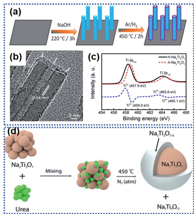
Fig. 4 Examples of creating surface oxygen vacancies in \text{Na}_2\text{Ti}_3\text{O}_7 : (a) schematic illustration of the preparation of hydrogen-reduced \text{Na}_2\text{Ti}_3\text{O}_7 ( \text{H-Na}_2\text{Ti}_3\text{O}_7 ), (b) TEM image of \text{H-Na}_2\text{Ti}_3\text{O}_7 , and (c) Ti 2p XPS spectra of air-treated \text{Na}_2\text{Ti}_3\text{O}_7 ( \text{A-Na}_2\text{Ti}_3\text{O}_7 ) and \text{H-Na}_2\text{Ti}_3\text{O}_7 (the blue dashed line represents the difference between the two XPS spectra). 68 Copyright 2016, American Chemical Society. (d) Schematic illustration of formation of surface OVs on \text{Na}_2\text{Ti}_3\text{O}_7 by reaction with urea in a nitrogen atmosphere at 450^\circ\text{C} . 67 Copyright 2021, Wiley-VCH.
