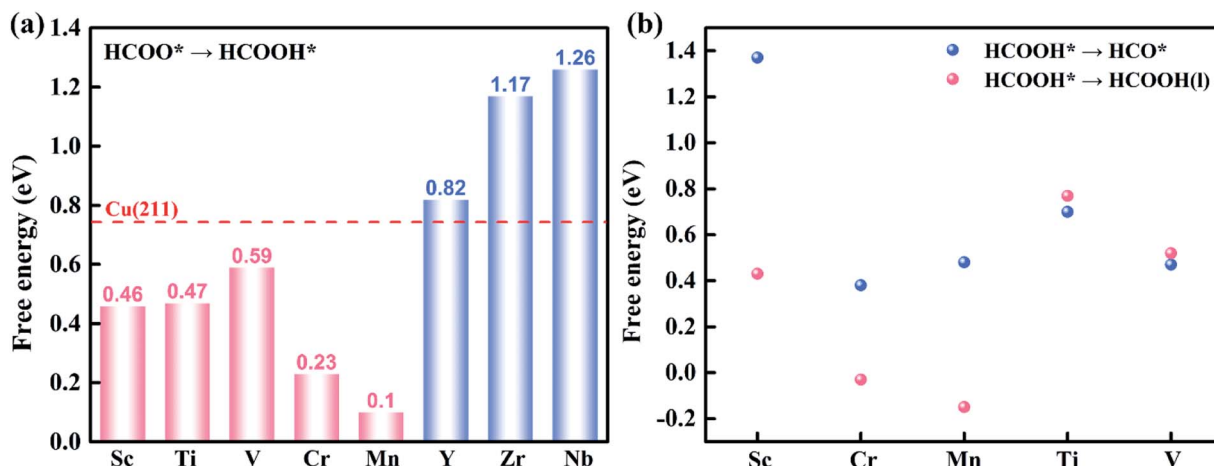
Fig. 5 (a) The \Delta G of \text{HCOO}^* + \text{e}^- + \text{H}^+ \rightarrow \text{HCOOH}^* on \text{TM@Na}_4\text{SiMo}_{12} ( \text{TM} = \text{Sc, Ti, V, Cr, Mn, Y, Zr} and \text{Nb} ). The screening criterion for catalytic activity is set to \Delta G < 0.74 eV (red dashed line). (b) The \Delta G for \text{HCOOH}^* hydrogenation ( \text{HCOOH}^* + \text{e}^- + \text{H}^+ \rightarrow \text{HCO}^* + \text{H}_2\text{O}(\text{l}) ) and desorption ( \text{HCOOH}^* \rightarrow \text{HCOOH}(\text{l}) + * ) on \text{TM@Na}_4\text{SiMo}_{12} ( \text{TM} = \text{Sc, Cr, Mn, Ti} and \text{V} ).
