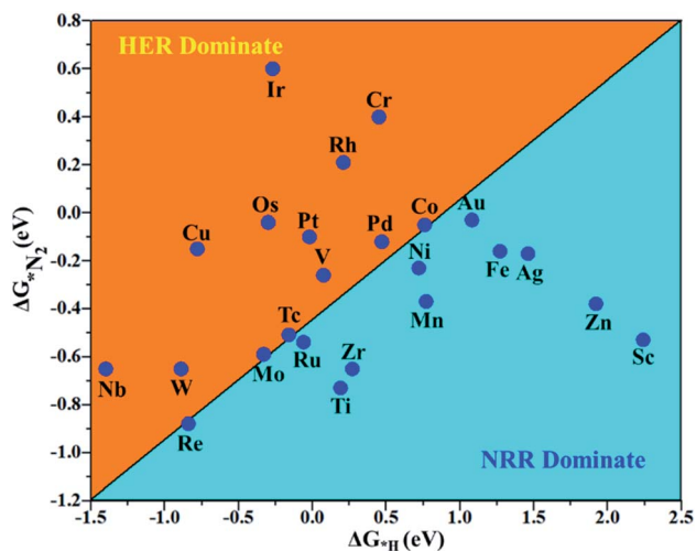
Fig. 4 Calculated Gibbs free energies of N_2 and H_2 adsorbed on the M_1 /PMA cluster, which are divided into the eNRR region ( \Delta G_{*H} > \Delta G_{*N_2} ) and HER region ( \Delta G_{*H} < \Delta G_{*N_2} ).
