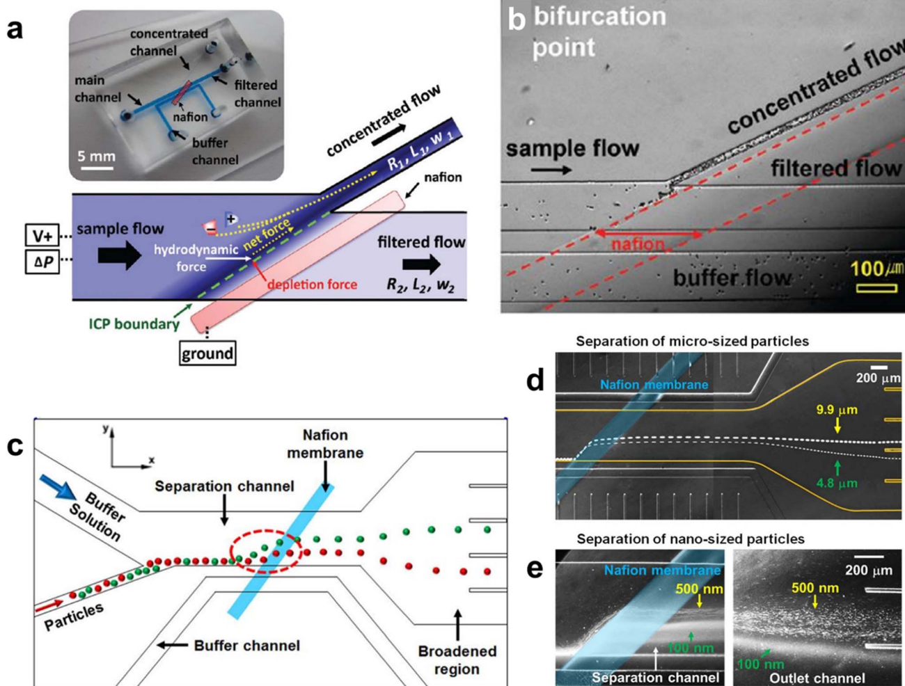
Fig. 1 (a) Schematic illustration and image of a microfluidic device designed to utilize ICP for continuous separations. (b) Micrograph showing the channel bifurcation of the device in (a) during operation. (a and b) Adapted from: Anal. Chem. , 2011, 83 , 7348–7355 (copyright © 2011 American Chemical Society). (c) Schematic illustration of the microfluidic device designed to continuously separate microplastics. (d and e) Micrographs of the device shown in (c) when separating different sizes of microplastics. (c–e) Adapted from Sci. Rep. , 2013, 3 , article number: 3483 (copyright © 2013 Nature Publishing Group).
