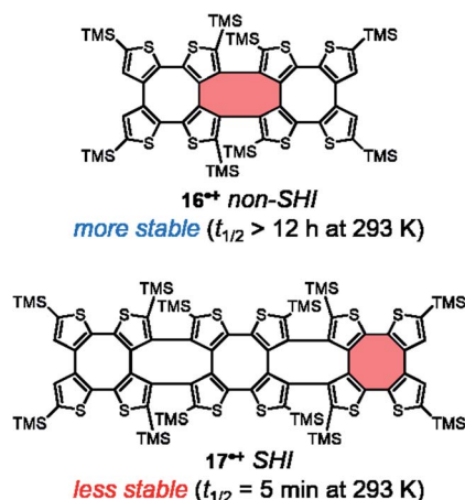
Fig. 14 Chemical structures of thiophene-based double helix radicals 16 and 17 + (TMS = trimethylsilyl). The molecular fragment in red highlights the predominant localization of the SOMO within the molecular structure.
