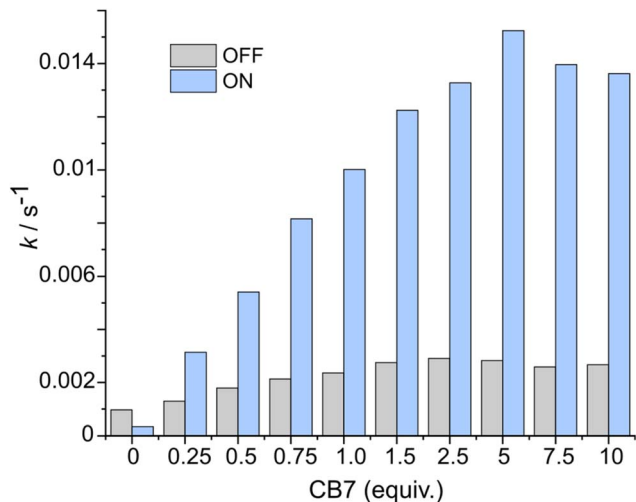
Fig. 3 Comparison of the rates of the hydrazone of the axle (75 \mu M) at different amounts of CB7 in the dark (grey bars) and under constant light irradiation (blue bars), acetonitrile/H 2 O mixture (v/v \approx 40 : 60), pH \approx 3, 298 K. The determination of the rates is described in pp. S34–S35, ESI † .
