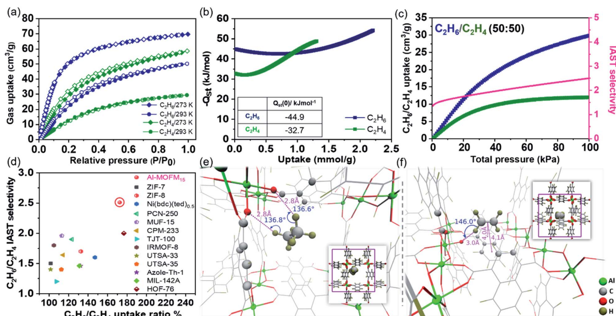
Fig. 1 (a) Single-component adsorption-desorption isotherms of C 2 H 6 and C 2 H 4 in Al-MOFM 15 measured at 273 and 293 K for pressures 0–690 torr. (b) Isothermic heats of adsorption ( Q_{\text{st}} ) of C 2 H 6 and C 2 H 4 at various loading amounts (near-zero coverage Q_{\text{st}} values are provided in the inset). (c) Mixed adsorption isotherms and selectivity calculated using IAST for C 2 H 6 /C 2 H 4 (50 : 50) in Al-MOFM 15 at 293 K. (d) C 2 H 6 /C 2 H 4 separation performance in some benchmark porous materials. (e and f) Locations of the highest binding affinity sites determined by DFT optimization for C 2 H 6 ( -39.9 \text{ kJ mol}^{-1} ) and C 2 H 4 ( -38.7 \text{ kJ mol}^{-1} ). Insets: Corresponding molecule locations, zoomed out, within the large channel. C 2 H 6 participates in two hydrogen-bonding interactions with carboxylate oxygens while C 2 H 4 participates in \pi - \pi and hydrogen-bonding interactions with the naphthalene ring and carboxylate oxygen, respectively. Binding sites with lower affinities for C 2 H 4 and C 2 H 6 are shown in Fig. S23 and S24,† respectively.
