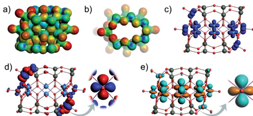
Fig. 15 Molecular electrostatic potential (MEP) plotted over the density isosurface of [V 10 As 12 O 40 ] 4- shown in (a) side and (b) top view. The most negative potentials are shown in red. Spin density isosurfaces indicating accumulation of \alpha spins for [V 10 As 12 O 40 ] 4- (c). Depiction of the HOMO (d) and the LUMO of [V 10 As 12 O 40 ] 4- (e). Colour code: V = blue, O = red, and As = green spheres.
