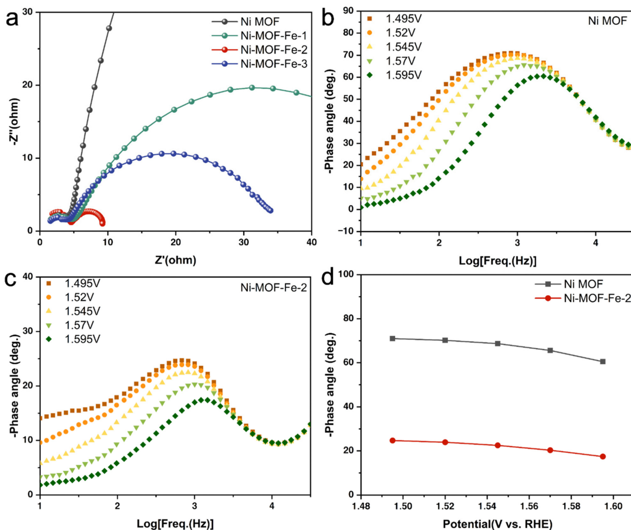
Fig. 4 (a) Nyquist plots of the catalysts at the potential of 1.52 V (vs. RHE). Bode plots of (b) Ni MOF and (c) Ni-MOF-Fe-2 obtained under different potentials. (d) Potential dependence of the phase angle of Ni MOF and Ni-MOF-Fe-2.
