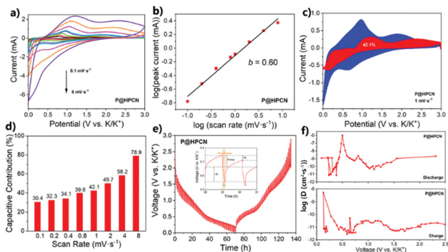
Fig. 4 (a) CV profiles of P@HPCN at various scan rates. (b) The corresponding b value plot. (c) The portion of capacitive contribution (red) in P@HPCN at a scan rate of 1 \text{ mV s}^{-1} . (d) The plot of capacitive contribution in P@HPCN with respect to various scan rates. (e) The GITT profiles for P@HPCN in the discharge and charge processes. (f) The diffusion coefficients of potassium ions for P@HPCN.
