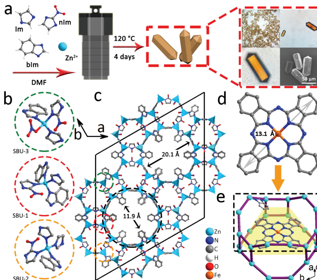
Fig. 1 (a) The route to prepare BMM-14 single crystals and their optical/SEM images; (b) three different Zn-based SBUs; (c) the cell unit; (d and e) FePc molecule and its encapsulation in a MOF cavity.
