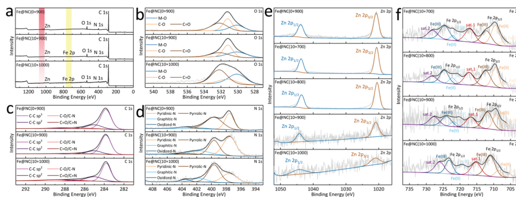
Fig. 5 (a) Full XPS survey spectra; the deconvoluted (b) O 1s, (c) C 1s and (d) N 1s of Fe@NC(0+900) and Fe@NC(10+y); the deconvoluted (e) Zn 2p and (f) Fe 2p of Fe@NC(0+900) and Fe@NC(10+y).
