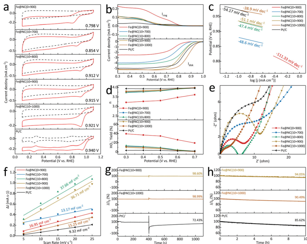
Fig. 6 (a) CV curves, (b) LSV curves, (c) Tafel slopes, (d) n and \text{HO}_2^- yields, (e) EIS plots, (f) C_{\text{dl}} values for \text{Fe@NC}(x+y) series and Pt/C; (g) anti-MeOH test, and (h) current retention for \text{Fe@NC}(10+900/1000) and Pt/C.
