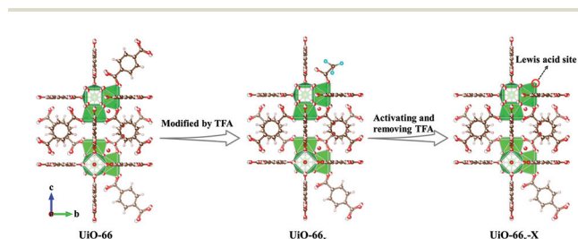
Fig. 1 Schematic illustration of the synthesis of UiO-66 x -X.
