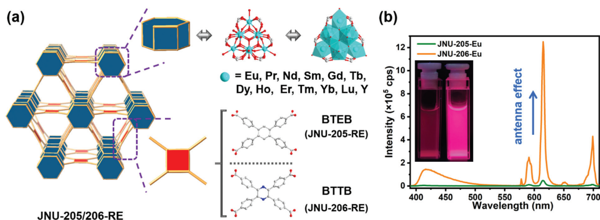
Fig. 1 (a) Crystal structure of JNU-205-RE / JNU-206-RE and tiling representation of the shp topology built from a 12-connected RE 9 -cluster and a 4-connected BTEB/BTTB linker (sky blue for RE, red for O, gray for C and blue for N; H atoms are omitted for clarity). (b) Comparison of emission spectra of aqueous suspensions of JNU-205-Eu and JNU-206-Eu (30 mg per 100 mL, \lambda_{\text{ex}} = 365 nm, slit = 1 nm). Inset: photographs of aqueous suspensions of JNU-205-Eu (left) and JNU-206-Eu (right) under 365 nm UV lamp.
