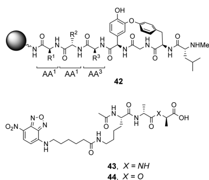
Fig. 16 Schematic of biomimetic combinatorial library 42 generated on ArgoGel TM resin beads and fluorescent NBD-labelled substrates 43 and 44 .
