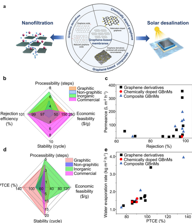
Fig. 1 (a) Schematic illustration of membranes prepared from graphene derivatives, chemically doped graphene, and graphene-based composites for NF and SD applications. Figure of merit comparing processability, economic feasibility, stability, and performance factors of (b) NF among various membrane materials and (c) upper-bound graph of NF. Figure of merit comparing processability, economic feasibility, stability, and performance of (d) SD among various membrane materials and (e) upper bound graph of SD.
