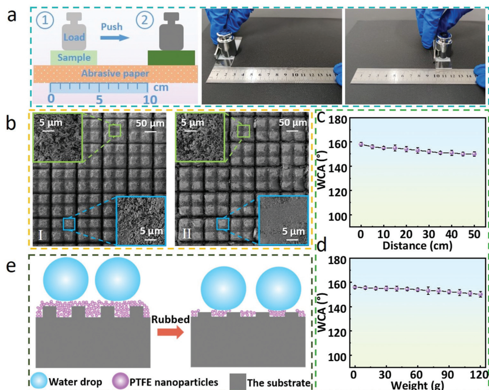
Fig. 5 (a) Schematic illustration and experimental diagram of the sandpaper friction test; (b) SEM images of the laser-treated glass surface before and after the friction; an enlarged view of a groove is shown in the upper left corner and an enlarged view of a protrusion is shown in the lower right corner; (c) the WCAs of various friction distances of laser-treated glass loaded with 50 g; (d) the change of WCAs on the laser-treated glass with a friction distance of 10 cm with the different load weights; and (e) schematic illustration of the principle that the laser-treated samples after friction still have superhydrophobicity.
