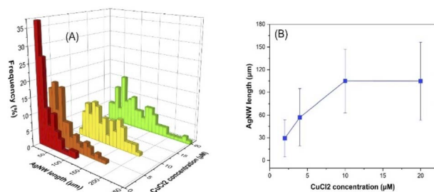
Fig. 7 Influence of \text{CuCl}_2 concentration on the AgNW length distribution (A) and the average length of the nanowires (B).
