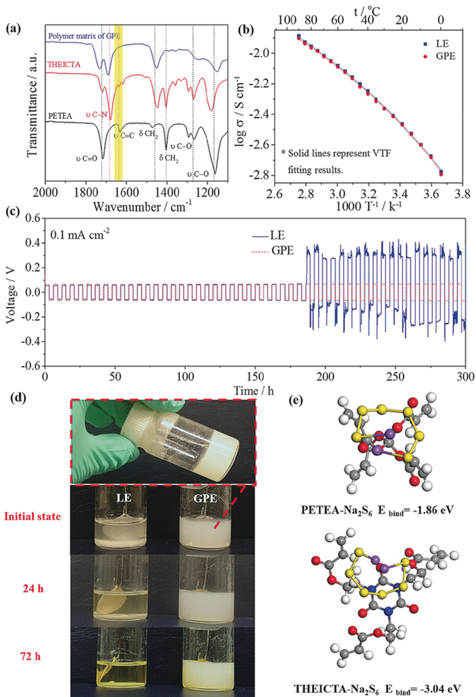
Fig. 12 Characterization and electrochemical performance of quasi-solid state electrolyte/GPE. (a) Overlaid FTIR spectra of polymer matrix and monomers showing the conversion of polymer to a monomer, (b) comparison of temperature-dependent ionic conduction of GPE and its liquid counterpart, (c) Galvanostatic cycling measurement (at a current density of 0.1 \text{ mA cm}^{-2} ) on a symmetric Na/Na cell with GPE and LE, (d) photographs showing the formation of sodium polysulfides and their dissolution in LE and its comparison with GPE at various times, and (e) binding energy calculation and the molecule bonded with \text{Na}_2\text{S}_6 , from first principles calculations. 220
