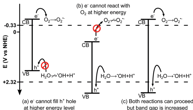
Fig. 6 Schematic illustration of redox potential for \text{•OH} and \text{O}_2^{\bullet -} showing (a) a semiconductor with sufficiently negative CB to allow \text{O}_2 + \text{e}^- , but VB too negative to allow \text{H}_2\text{O} + \text{h}^+ as \text{H}_2\text{O} cannot donate an electron to fill the more negative hole in the VB of the semiconductor. (b) A semiconductor with sufficiently positive VB such that \text{H}_2\text{O} may donate an electron to fill the hole, however the CB is too positive meaning \text{O}_2 cannot accept \text{e}^- . (c) A semiconductor with both a sufficiently negative CB, and a sufficiently positive VB. This semiconductor would be capable of facilitating both reactions but has an increased band gap, limiting its solar spectrum adsorption range. Heterojunctions (Fig. 7) can be used to reduce this band gap whilst maintaining the redox potentials. Figure is for illustrative purposes only and is not drawn to scale.
