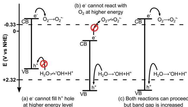
Fig. 6 Schematic illustration of redox potential for \cdot OH and O_2^{\cdot -} showing (a) a semiconductor with sufficiently negative CB to allow O_2 + e^- , but VB too negative to allow H_2O + h^+ as H_2O cannot donate an electron to fill the more negative hole in the VB of the semiconductor. (b) A semiconductor with sufficiently positive VB such that H_2O may donate an electron to fill the hole, however the CB is too positive meaning O_2 cannot accept e^- . (c) A semiconductor with both a sufficiently negative CB, and a sufficiently positive VB. This semiconductor would be capable of facilitating both reactions but has an increased band gap, limiting its solar spectrum adsorption range. Heterojunctions (Fig. 7) can be used to reduce this band gap whilst maintaining the redox potentials. Figure is for illustrative purposes only and is not drawn to scale.
