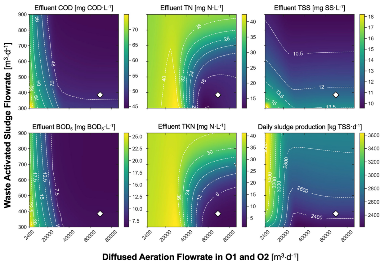
Fig. 6 Effluent quality metrics mapped across the decision space of aeration and sludge waste. The diffused aeration air flowrate at field condition in the first two aerated CSTRs (i.e., O1 and O2) was varied uniformly between 2400 \text{ m}^3 \text{ d}^{-1} and 86765 \text{ m}^3 \text{ d}^{-1} , corresponding to a K_{La} of 80\text{--}300 \text{ d}^{-1} . The WAS flowrate was varied uniformly within 300\text{--}900 \text{ m}^3 \text{ d}^{-1} , resulting in an SRT of 4.15\text{--}17.2 days. The white diamonds represent the baseline setting.
