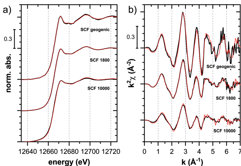
Fig. 8 Tl L_{III} -edge (a) XANES and (b) EXAFS spectra of a soil clay fraction (SCF) with \sim 260 \text{ mg kg}^{-1} geogenic Tl (SCF geogenic) and with an additional 1800 \text{ mg kg}^{-1} (SCF 1800) or 10\,000 \text{ mg kg}^{-1} freshly adsorbed Tl (SCF 10000) (black lines) and linear fit reconstructions (red lines). LCF results are listed in Table 2.
