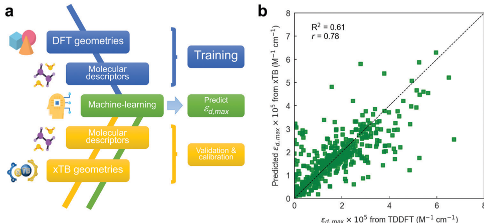
Fig. 5 (a) ML workflow used in this work to draw \epsilon_{d,max} predictions. A RF model is trained on TDDFT data and interpolated (validated) on xTB geometries, including also their corresponding molecular descriptors. To improve the accuracy of the model, energy levels obtained using the GFN2-xTB Hamiltonian require calibration with TDDFT values (Fig. S23, ESI † ). (b) Leave-one-out interpolation of the resulting RF model using three input molecular descriptors (including calibrated energy levels) and a 64-bit Morgan fingerprint vector.
