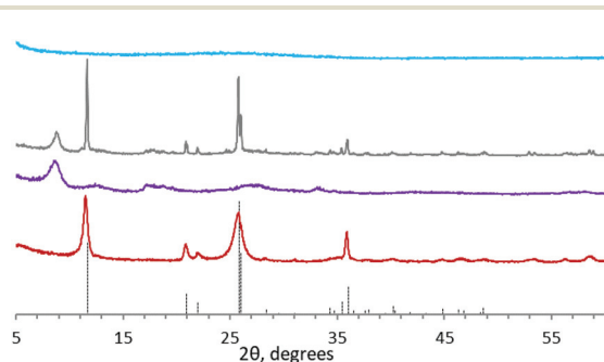
Fig. 2 Powder XRD patterns of the synthesised TiP products: \alpha TiP – sample 4, LTP-H – sample 3, TiP1-H – sample 1 and \alpha -TiP – sample 2 (adapted from ref. 35). The dotted line represents the referenced pattern of \alpha -TiP (ref. 4).
