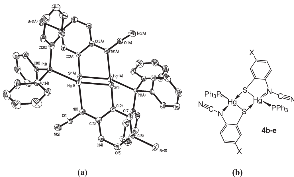
Fig. 3 (a) Molecular structure of [\text{Hg}\{\text{SC}_6\text{H}_3\text{BrN}(\text{C}\equiv\text{N})\}(\text{PPh}_3)_2] 4d . 8 Thermal ellipsoids are displayed at 50% probability and hydrogen atoms omitted for clarity. Selected bond lengths (Å) and bond angles (°): Hg1–N1 2.266(5), Hg1–S1 2.411(2), Hg1–S1A 2.871(2), Hg1–P1 2.272(2), N1–C1 1.287(8), N2–C1 1.154(8); Hg1–S1–Hg1A 83.57(5), S1–Hg1–S1A 96.43(5), S1–Hg1–N1 80.76(14), P1–Hg1–S1 151.40(6), P1–Hg1–N1 122.19(13), N1–C1–N2 174.6(7); (b) line drawing highlighting the bonding within 4b–e .
