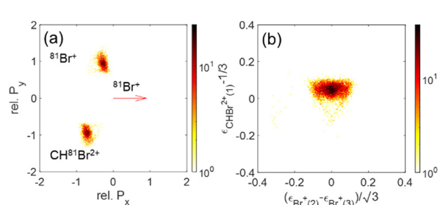
Fig. 13 (a) Newton plots of the Br + + Br + + CHBr 2+ channel with Br + as reference fragment. (b) Dalitz plot for the same fragmentation channel.
