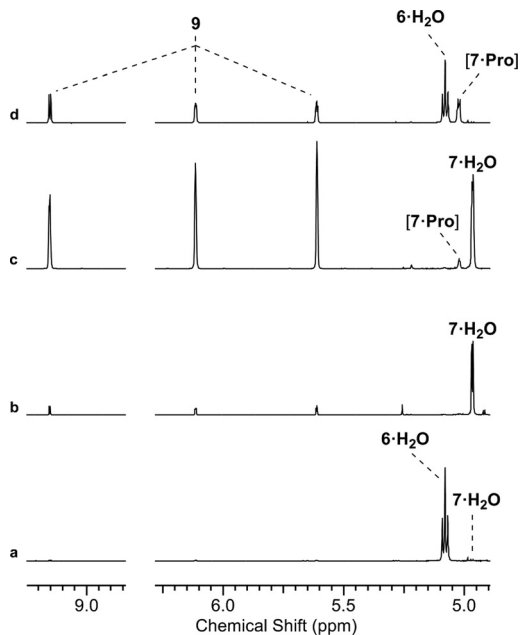
Fig. 3 Proline-catalysed aldol-elimination cascade. (a) 1 H NMR [400 MHz, noesygpprld, H 2 O/D 2 O (9 : 1)] spectrum to show the reaction of glycolaldehyde phosphate ( 6 , 100 mM) with formaldehyde ( 8 , 100 mM) in phosphate buffer (500 mM, pH 7) at 40 °C after 48 h; (b and c) 1 H NMR [700 MHz, noesygpprld, H 2 O/D 2 O (9 : 1)] spectra to show the reaction of glyceraldehyde-2-phosphate ( 7 , 100 mM) in phosphate buffer (500 mM, pH 7) with 50 mol% L-Pro at 40 °C after: (b) 0.5 h; (c) 48 h; (d) 1 H NMR [400 MHz, noesygpprld, H 2 O/D 2 O (9 : 1)] spectrum to show the reaction of 6 (100 mM) with 8 (100 mM) in phosphate buffer (500 mM, pH 7) with 50 mol% L-Pro at 40 °C after 7 h.
