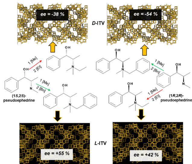
Fig. 1 Scheme of the synthetic route to the two enantiomeric crystalline polymorphs of the -ITV framework ( P 4 1 32 and P 4 3 32 space groups) by using the two derivatives of the enantiomers of pseudoephedrine through GTM-3 (by attachment of an ethyl group, red-arrows routes) or GTM-4 (by attachment of a benzyl group, green-arrows routes). D/L notation is arbitrary and does not mean an actual absolute configuration of the zeolite.
